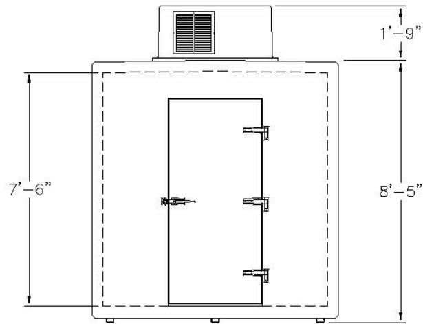
ELEVATION VIEW
